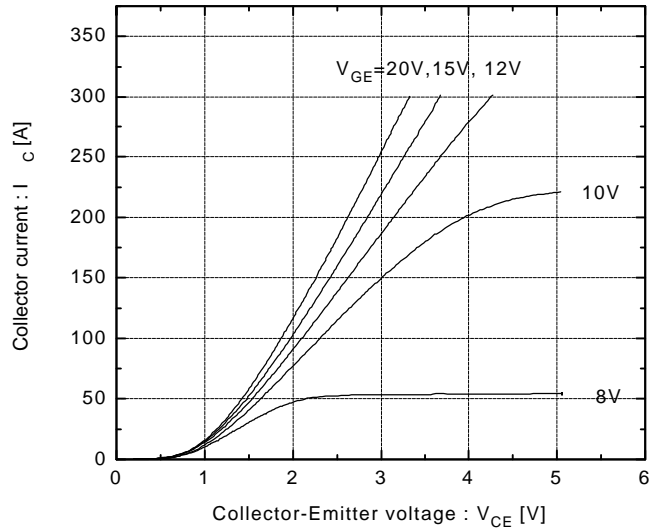
Collector current vs. Collector-Emmitter voltage T_j=125^\circ\text{C}
